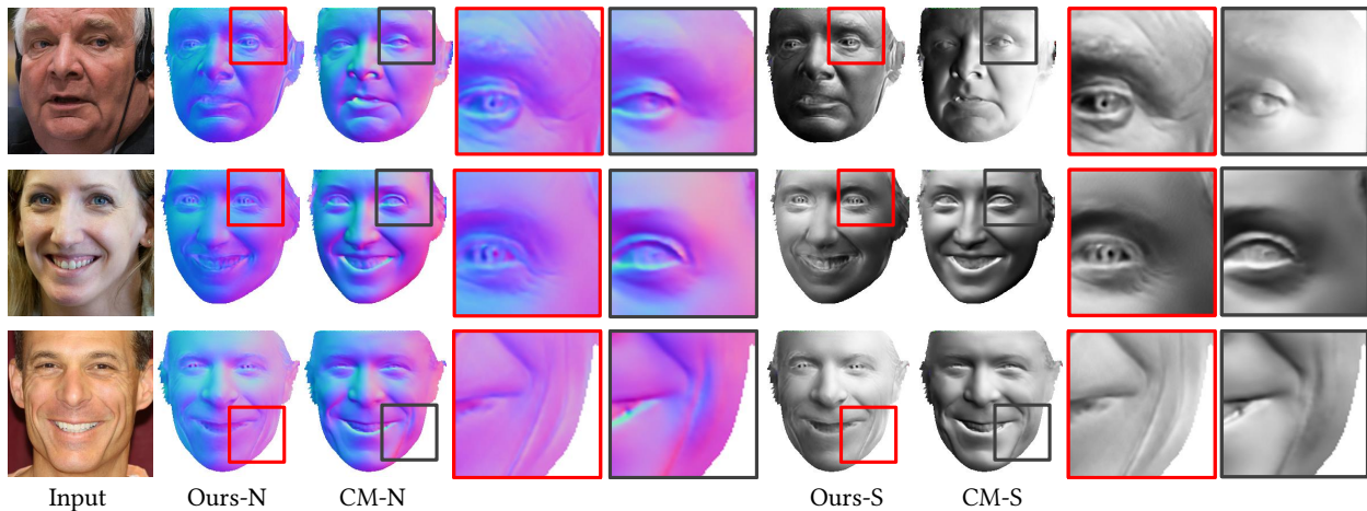
Figure 4: Comparisons in normal and geometric shading on the FFHQ [28]. We use different angles of light to render our geometric shading (Ours-S) and ‘Cross-modal’ [1] shading (CM-S) to exhibit more details.
