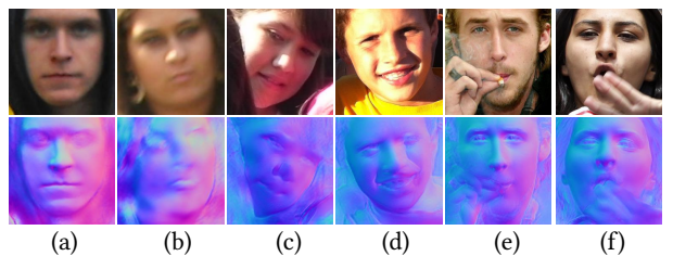
Figure 11: Results on low-quality, extreme lighting, and occluded faces.
