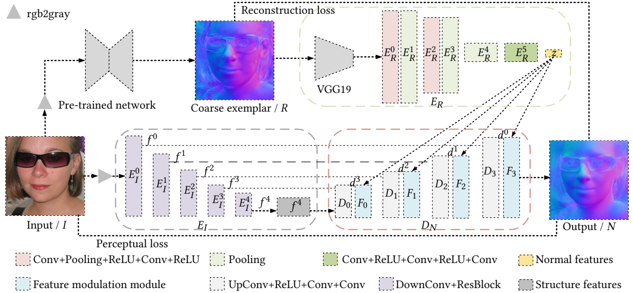
Figure 2: Illustration of our coarse-to-fine framework, which can produce high-fidelity normal via encoding the coarse exemplar normal into normal features together with the face structure features.
