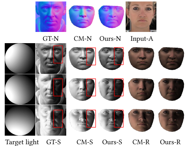
Target light GT-S CM-S Ours-S CM-R Ours-R Figure 7: Face relighting with estimated normal. ‘S’, ‘N’, ‘R’ and ‘A’ represent as shading, normal, and relighting and albedo, respectively.
